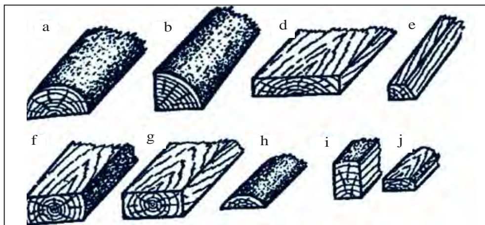
33-su'wret. Pishqi'lang'an materiallardin' u'lgileri: a) plastinka; b) shereklik; d) tazalap qi'rqi'lg'an taxta; e) sheti qi'rqi'lg'an reyka; f) yeki qi'rli' brus; g) tazalap qi'rqi'lg'an brus; h) u'sh qi'rli' brus; j) shpal.
